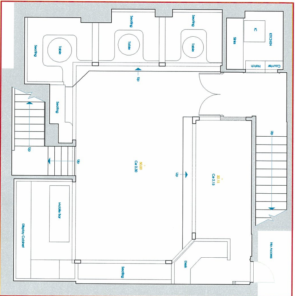
Proposed Lower Ground Floor Plan
